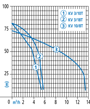
Aquabloc KV3/10T
