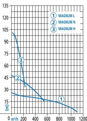
Grindex Magnum
