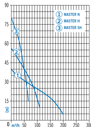
Grindex Master
