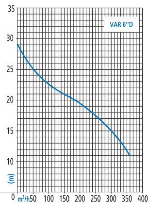
Varisco 6''D
