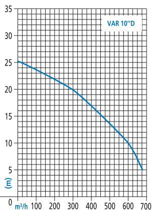
Varisco 10''D
