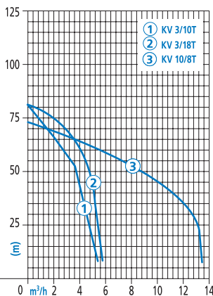
Aquabloc KV3/10T
