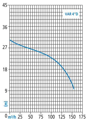
Varisco 4''D
