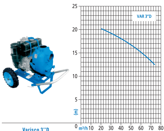
Varisco 3''D
