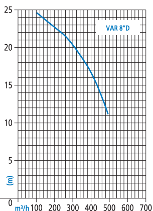
Varisco 8''D
