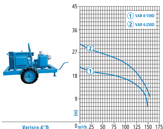
Varisco 4''D
