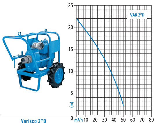
Varisco 2''D
