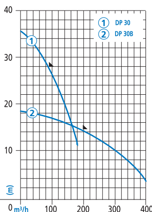
Toyo DP 30
